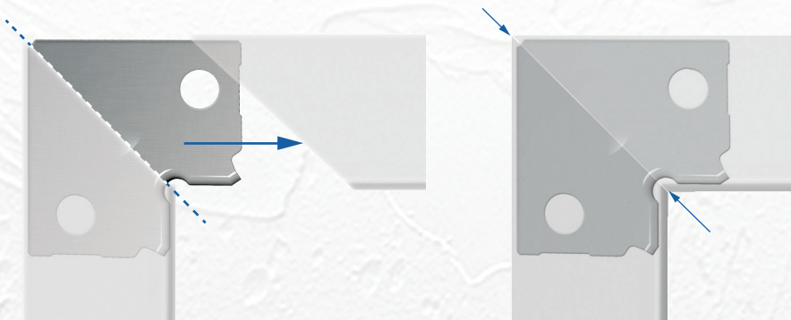
MiterGard is factory-attached to vertical casing. Exposed section slides securely into header casing
